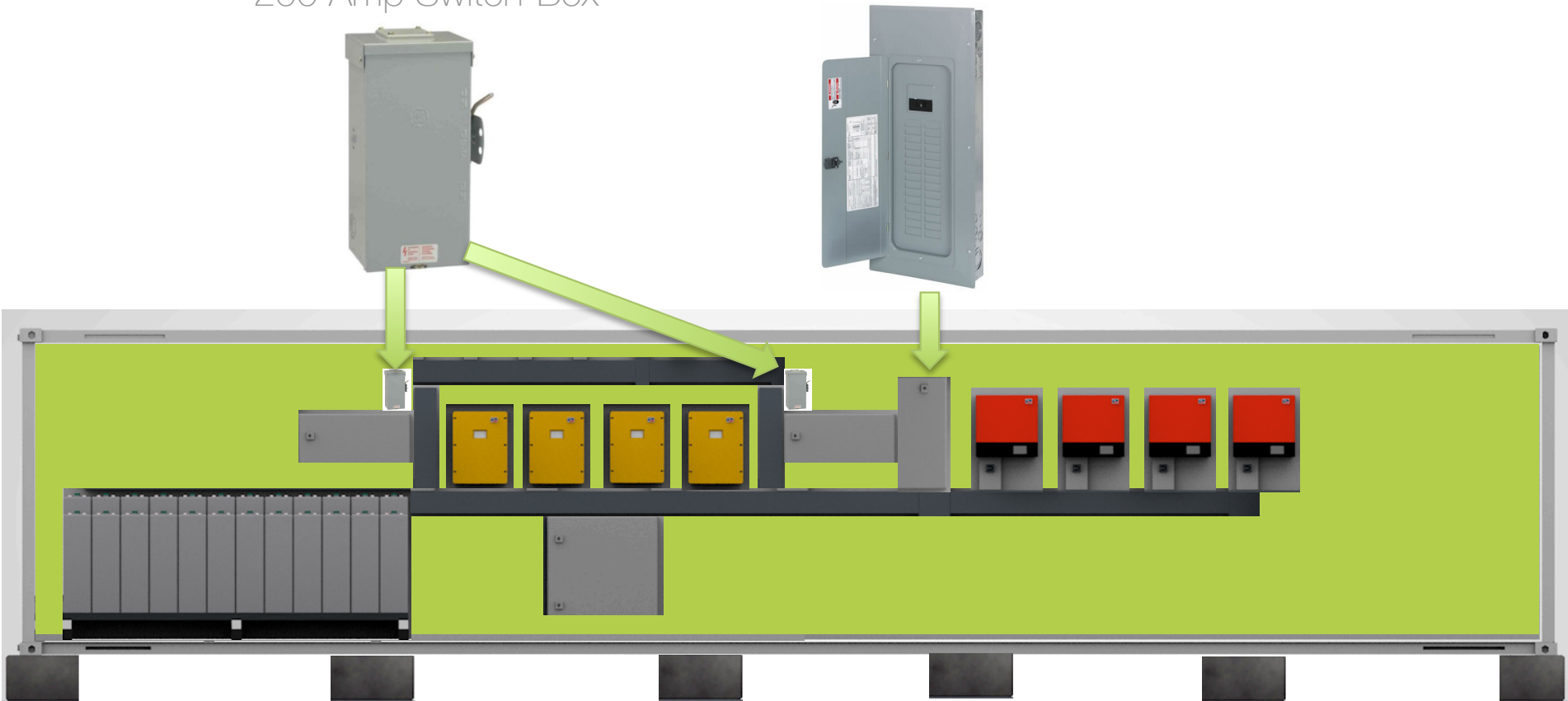
200 Amp Breaker-box
